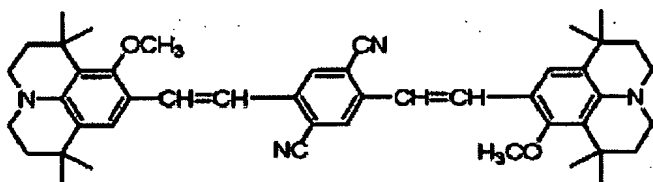
Structural formula (15)-9:
